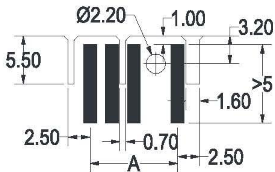
PCB Layout
